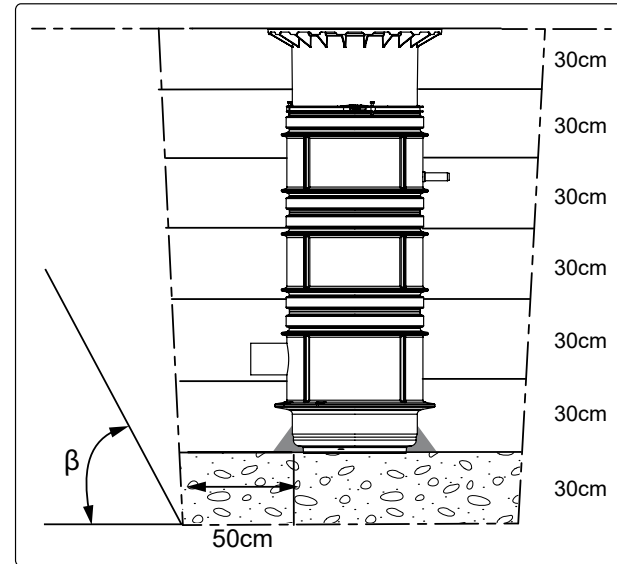
Abb. [6] Bodenaushub
