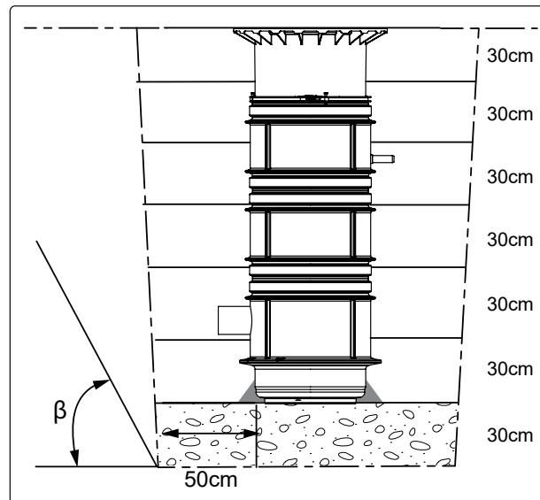
fig. [6] Excavation
